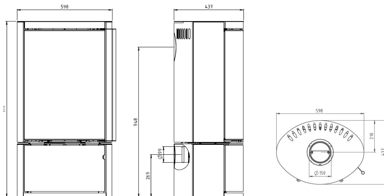
Figure 1 – Dimensions
