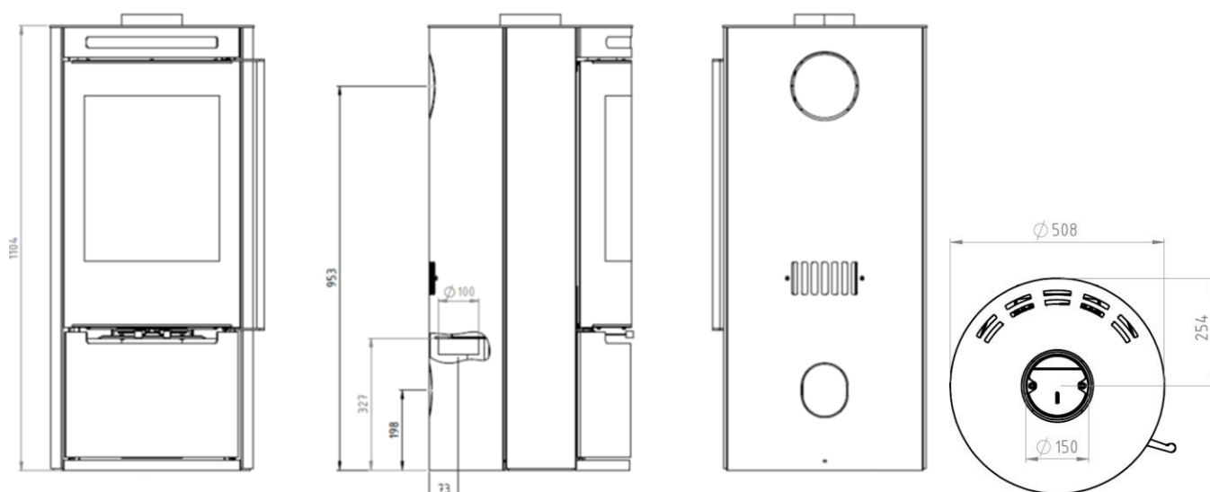
Figure 1 – Dimensions
